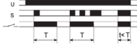
FZ06: Impulsformer
