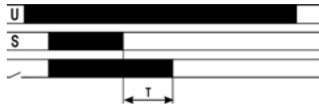
FZ73: Impulsformer
