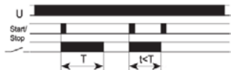
FZ38: On delay with Start/Stop pushbutton
