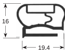
9200
