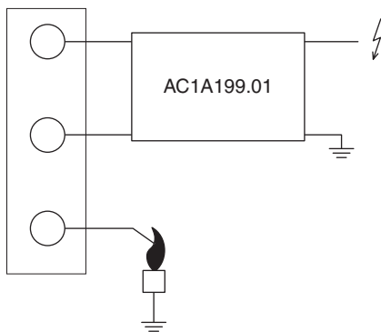
Fig. 50. Alternative side connection for external AC1A199.01 igniter
