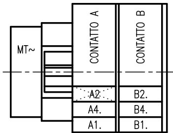
TIMER 120" (CROUZET 600 627/5261).
