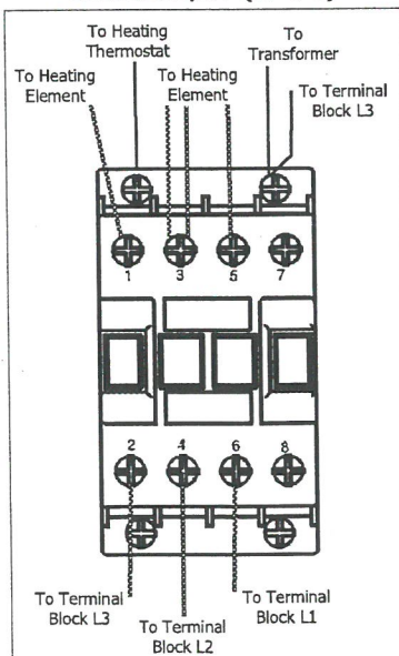
Heating Contactor E32SUBC3/C4 (3P + E)
