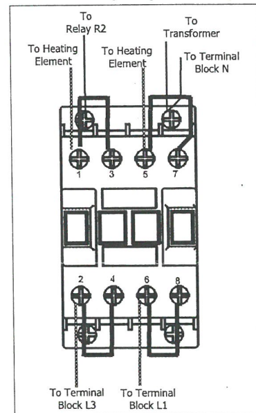
Heating Contactor E32SUBC3/C4 (3P + N + E)
